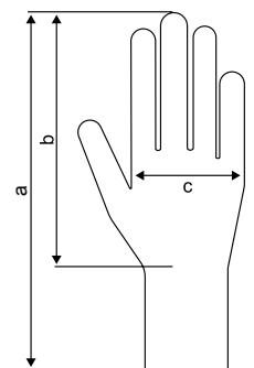
a= Total Glove Length b= Hand Length c= Peripheral Length
